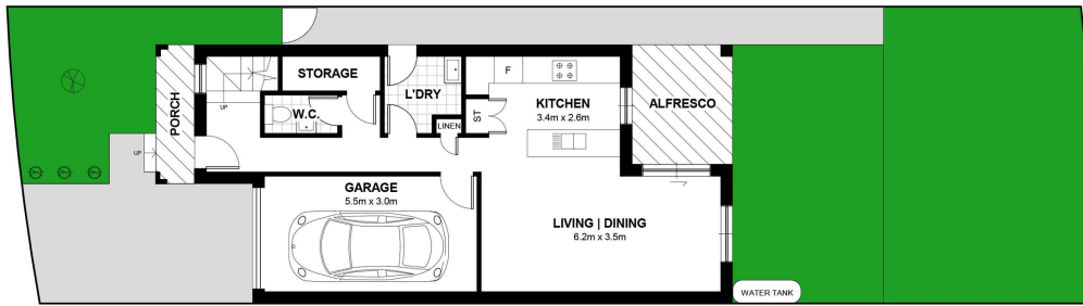
GROUND FLOOR
